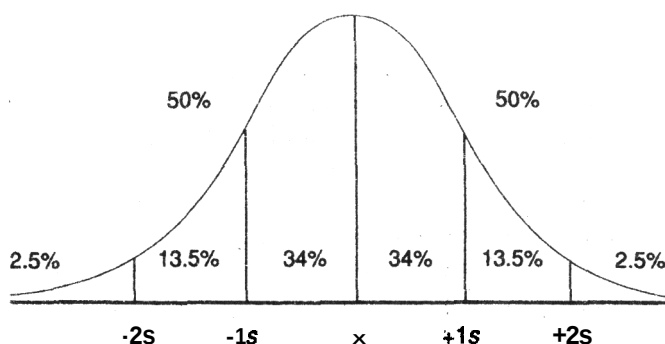
Figure 3.6 Some characteristics of normal distribution
